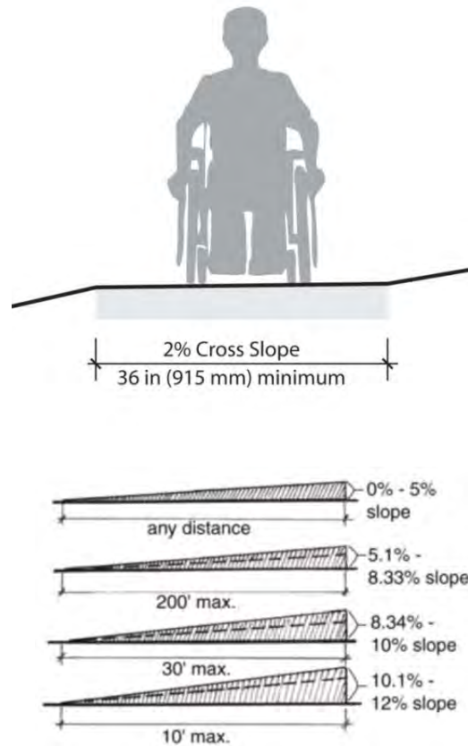
Trail gradients as recommended by the California State Parks Accessibility Guidelines
