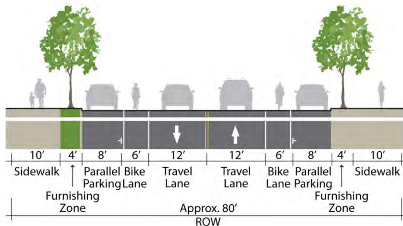
Figure 7-17: 4A Existing (Top) and Conceptual (Middle and Bottom) Cross Sections, Facing Northwest
