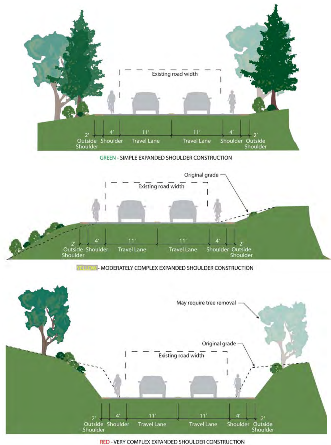
Figure 7-6: Conceptual Cross Sections Showing Cut and Fill Along SR 128 (Segment 2: Upper Valley)
