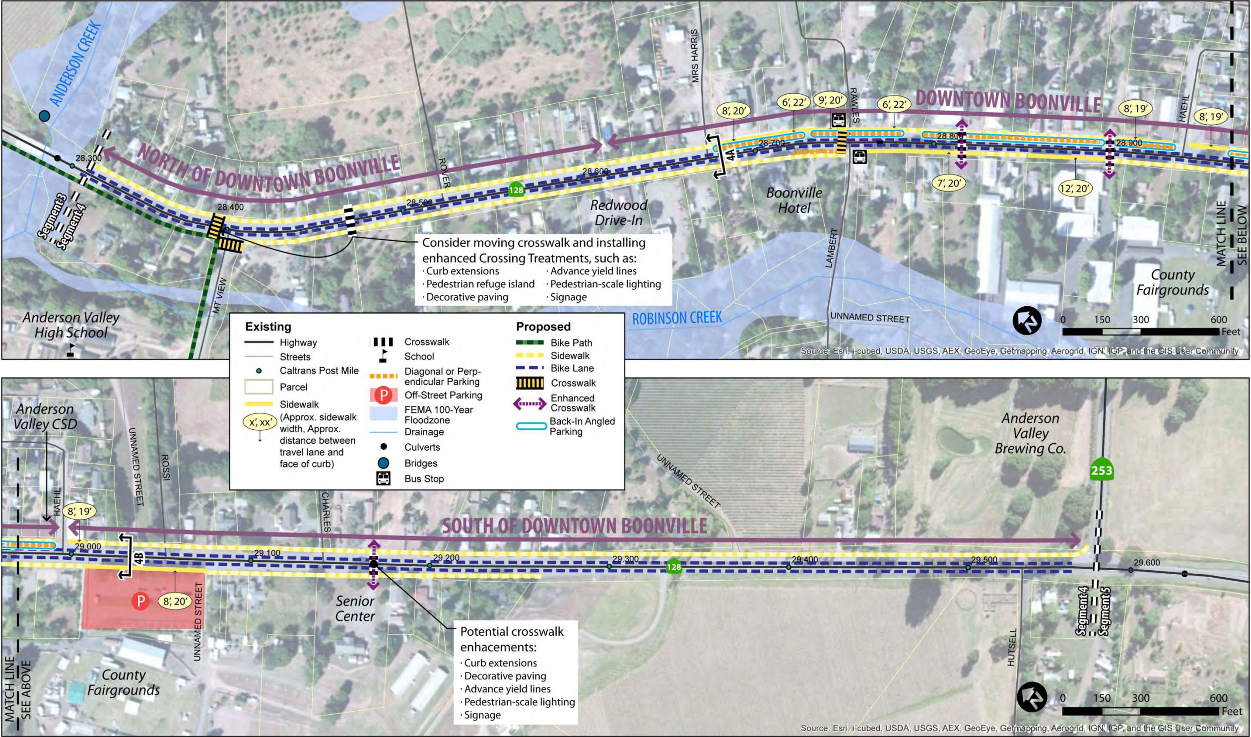
Figure 7-12: Segment 4 Central Boonville Design Concepts
