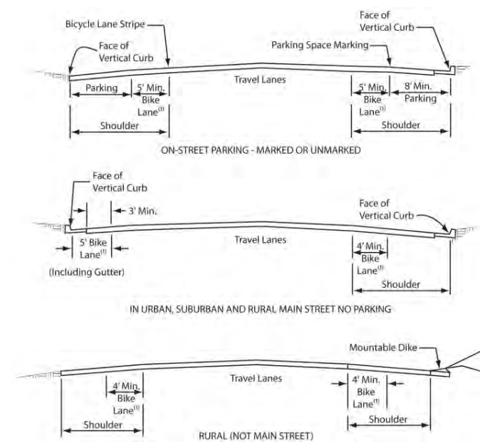
Caltrans Standards for Class II Bike Lanes on Rural Highways (Figure 301.2A)
