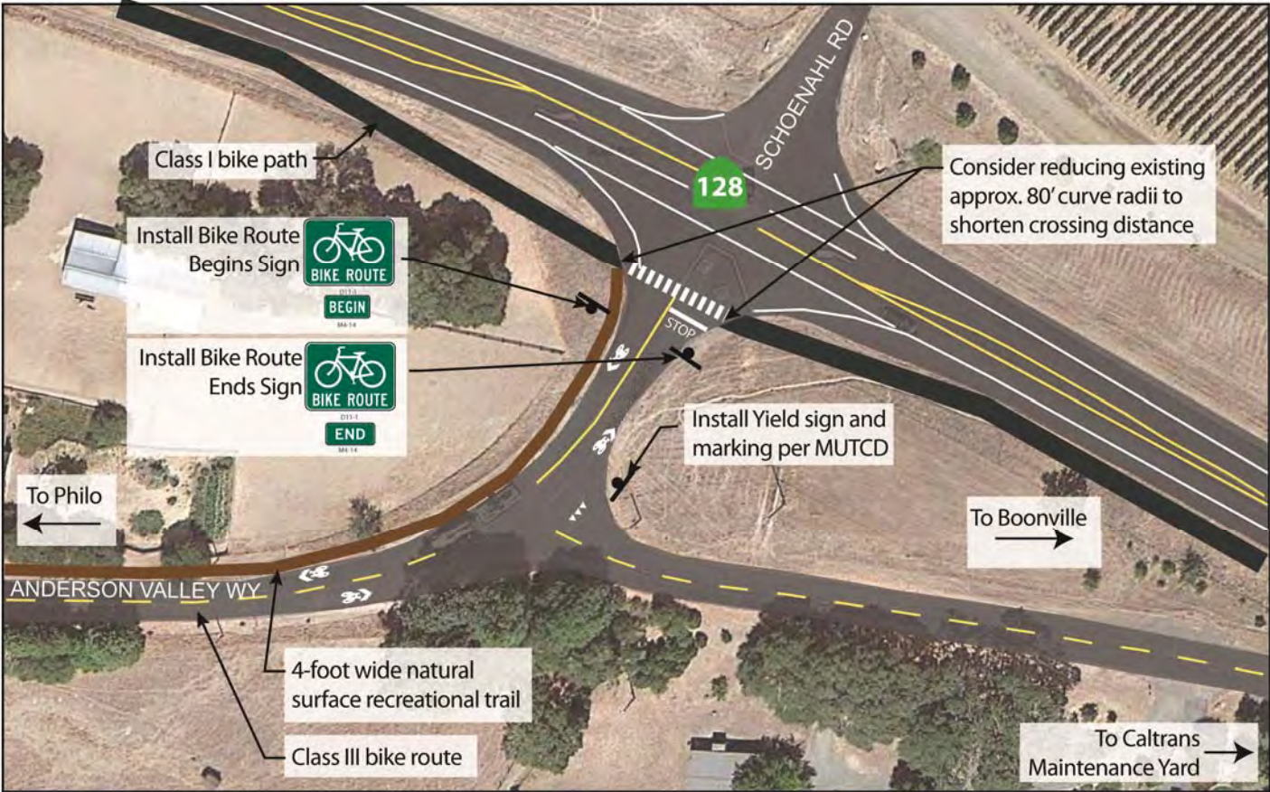
Figure 7-11: Southern Anderson Valley Way Entrance (Enlargement)
