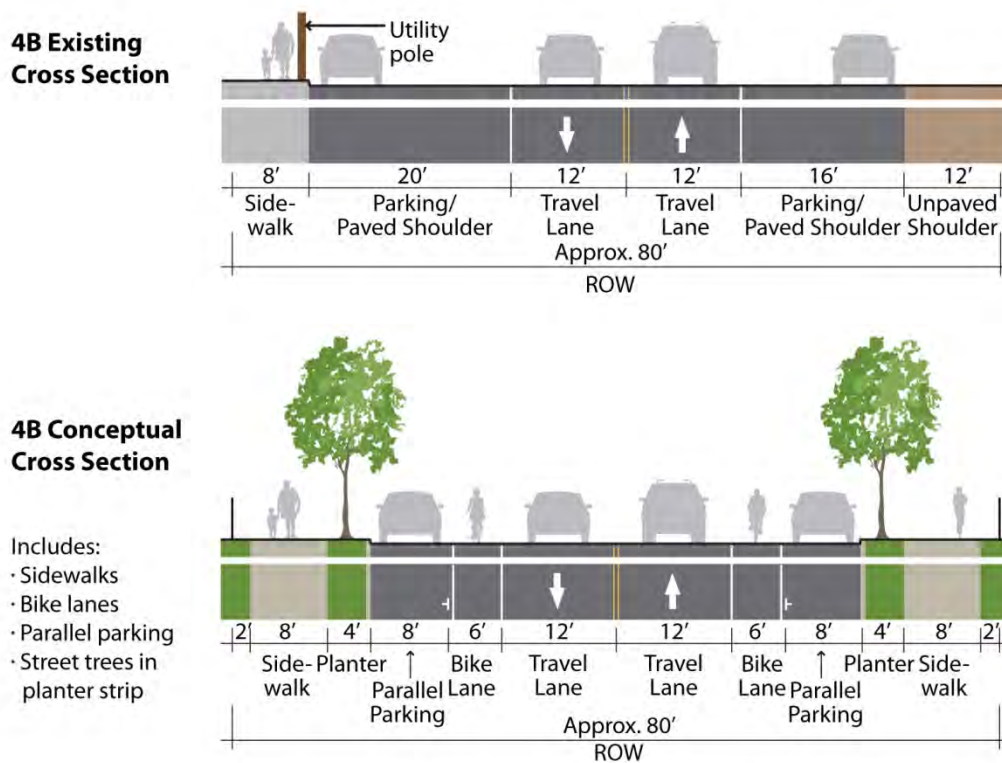
Figure 7-13: 4B Existing (Top) and Conceptual (Bottom) Cross Sections, Facing Northwest
