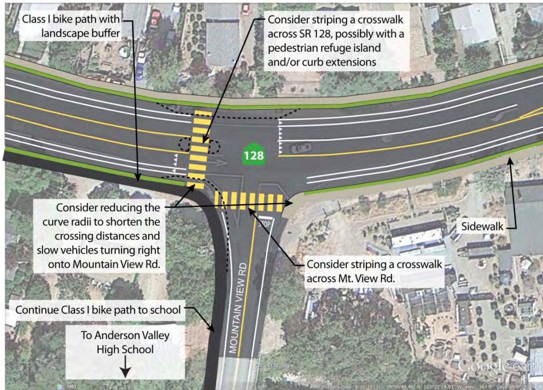
Figure 7-16: Conceptual Improvements to SR 128/Mt. View Road Intersection
