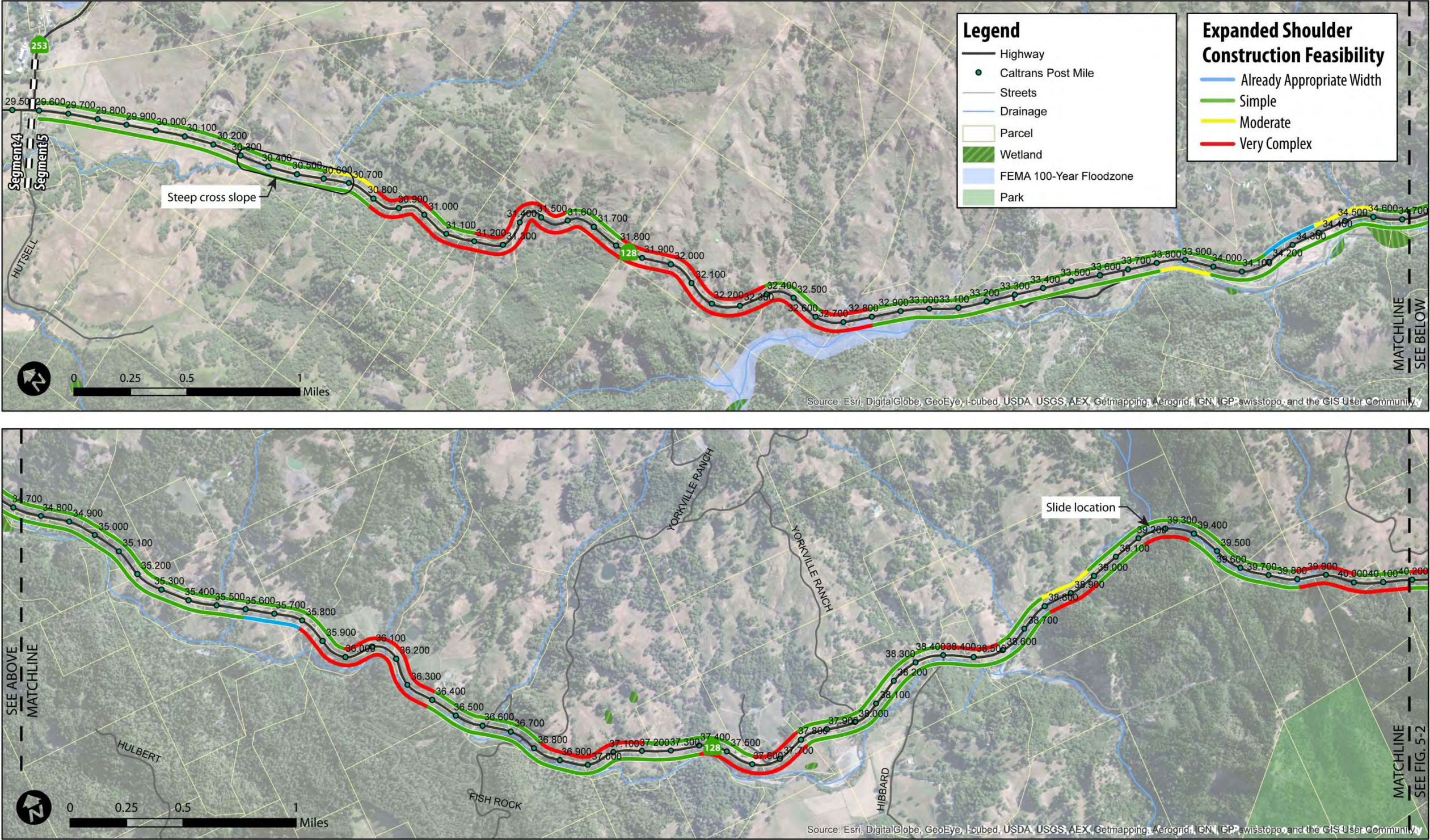
Figure 7-19: Segment 5 Hills and Valleys (West Half) – Design Concepts
