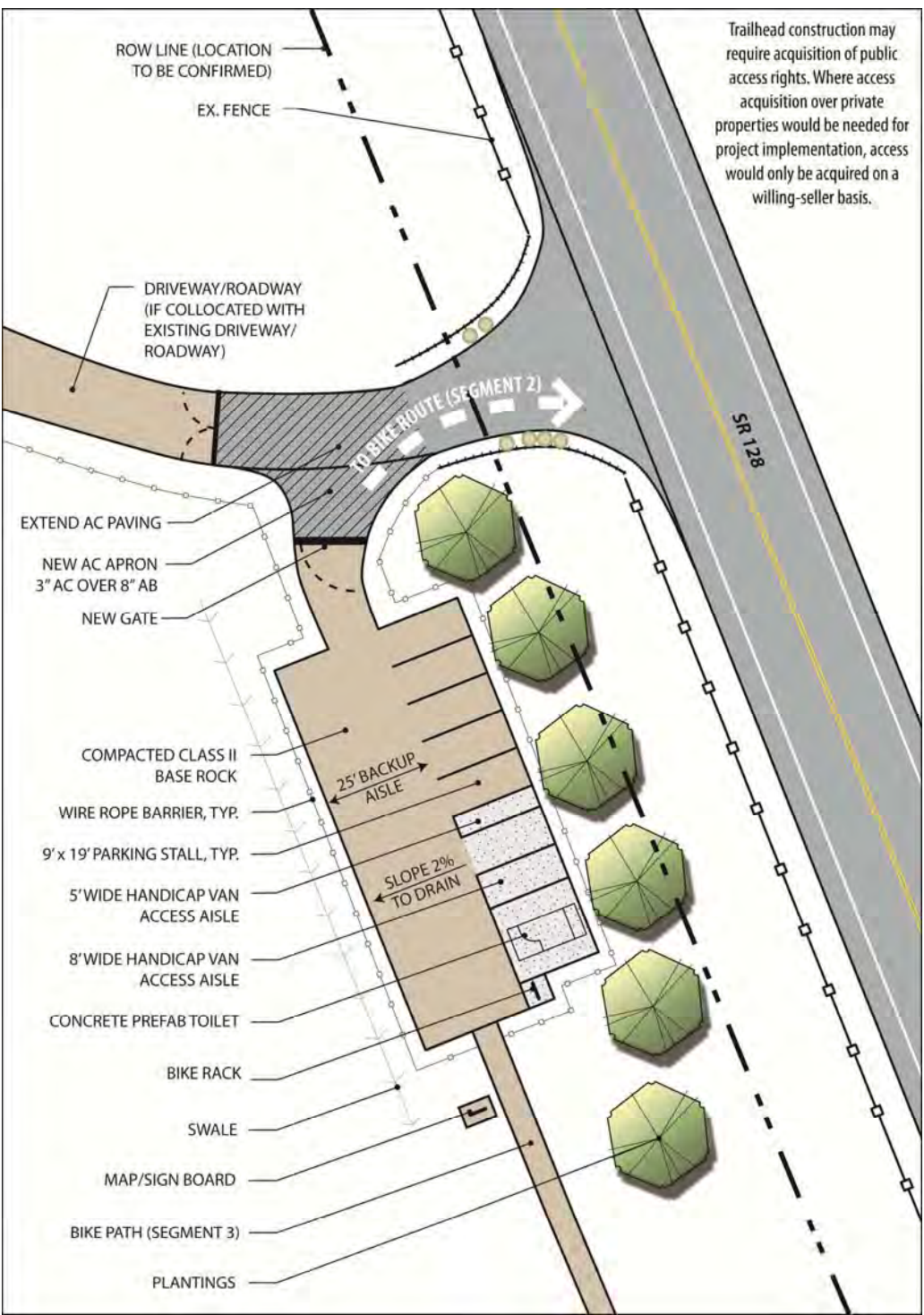
Figure 7-7: Conceptual Major Trailhead (Location To Be Determined)
